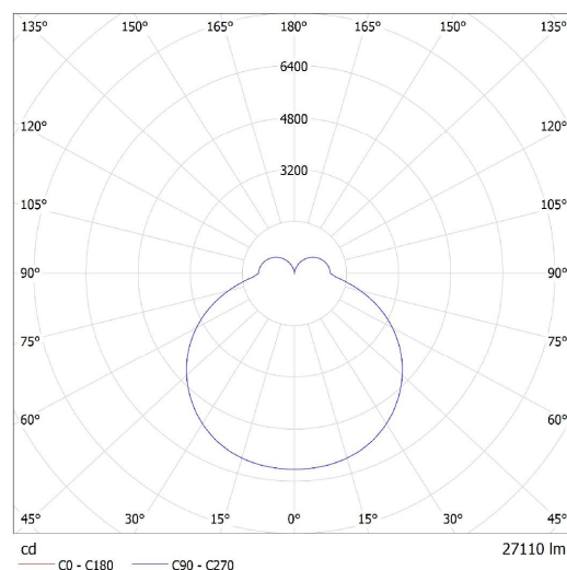
Lucis IB.L12.1250M.1 IZAR B MAX LED / LDC (Polar)
